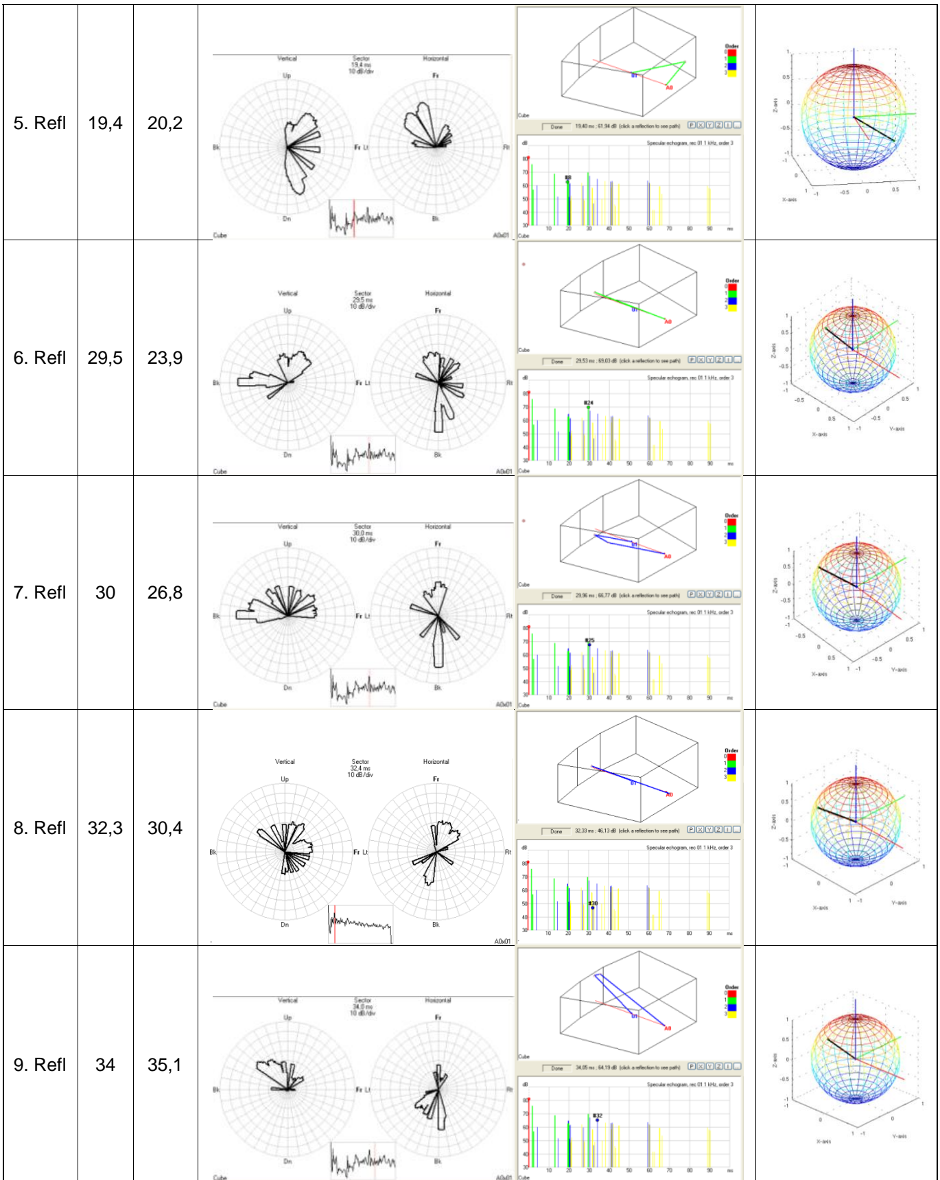
Figure 4.37: Graphical Comparison of the Simulation and the Real Measurement of the Detected Directions from the Direct Sound up to the 9 th Detected Reflection of the Impulse Response of Loudspeaker Number 1 in the CUBE. (1 st column: detected sound events from the measurement (cf. Figure 4.36), 2 nd and 3 rd column: arise time in [ms] of the sound events, 4 th column: results of the simulation, 5 th column: results from the measurement)
