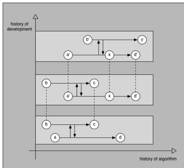
Figure 1: When modularizing the algorithm, a part can be exchanged without changing the temporal development of the other. Here, a pair of algorithms (visually connected by grey zones) is developed together: in a first step, x is inserted in ( ad ), while keeping ( bc ) the same. In a second step, ( bc ) is changed to ( b'y ), while keeping ( a'xd' ).
