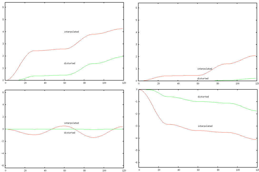
Figure 4: Phases of the ideal anti-/vortex ( upper figure ) and random configurations ( four lower figures ) for the XY sonification. The interpolated curves are depicted in red (and magenta), the distorted one according to Eq. 5 in green (and blue). The x-axis gives the number of samples. When the phase is looped, it is added smoothly to the last value, the base oscillation is periodic in 2\pi and does an effective modulo.)
